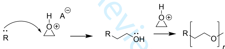
Scheme 12. Chain-initiation and chain-propagation steps in cation-activated-monomer polymerization of oxirane where the activator is a protic acid (AH)
