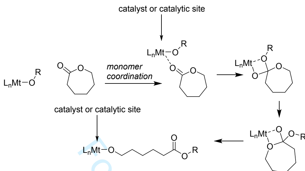
Scheme 20. Chain-propagation step in ring-opening coordination polymerization of caprolactone.
