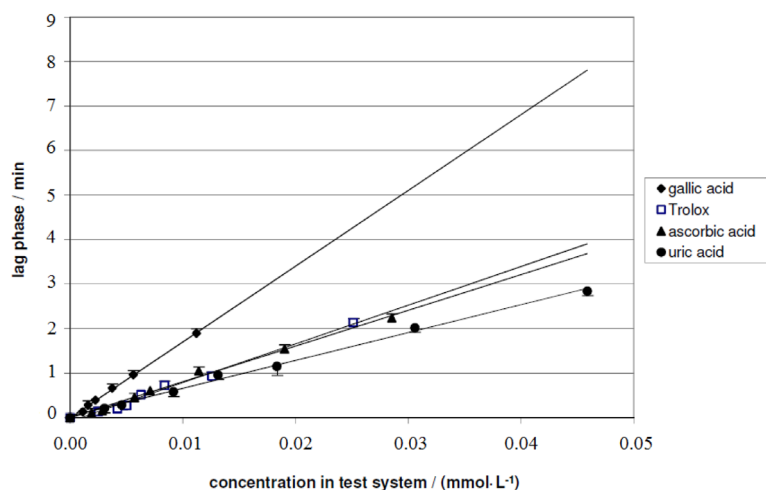
Fig. 1 Lag phases [min] of the four standard antioxidants; AA, gallic acid, Trolox, and uric acid, using different concentrations in the TEAC assay [10].
