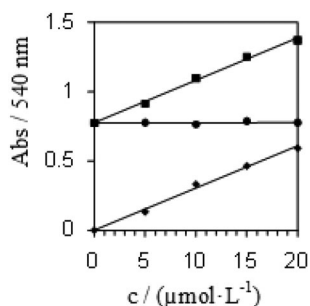
Fig. 6 Scavenging activity astaxanthin measured by DPPH assay [25]. ■ DPPH and astaxanthin; ◆ astaxanthin; ● differential curve of DPPH after subtracting absorbance of astaxanthin.
