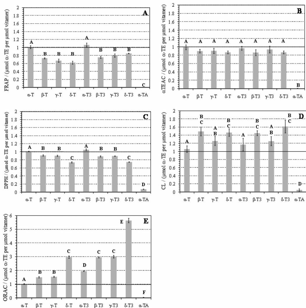
Fig. 5 Antioxidant activity of tocopherols, tocotrienols, and \alpha -tocopherol acetate measured by FRAP assay [A], \alpha TEAC assay [B], DPPH assay [C], CL assay [D], and ORAC assay [E]. Bars with different superscript letters differ significantly ( p < 0.05 ) [24].
