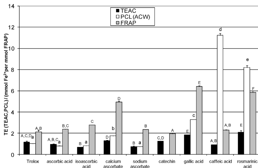
Fig. 3 Hydrophilic antioxidant activity of food additives and secondary plant products in the FRAP, TEAC, and PCL (ACW) assays. Bars for the same assay with different superscript letters are significantly different, p < 0.05 [21].
