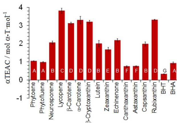
Fig. 7 Antioxidant activity of carotenoids as well as of BHT and BHA measured by \alpha TEAC assay. Bars with different letters differ significantly ( p < 0.05 ) [25].
