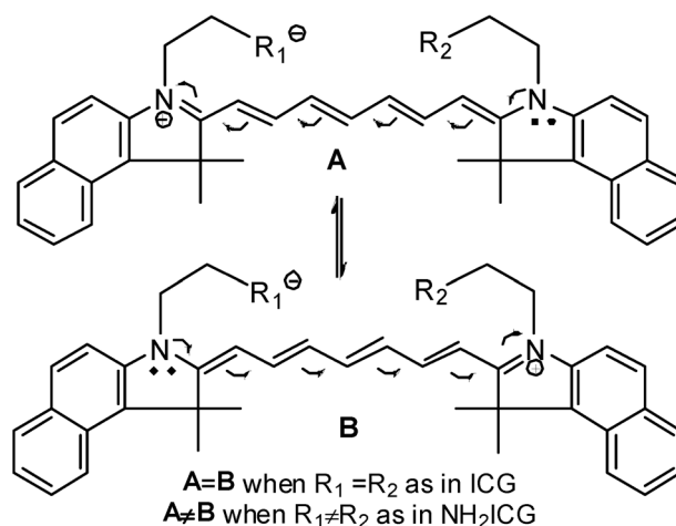
Fig. 3 Differentiation of functional groups causes non-equivalency in terms of charge location in resonance theory.
