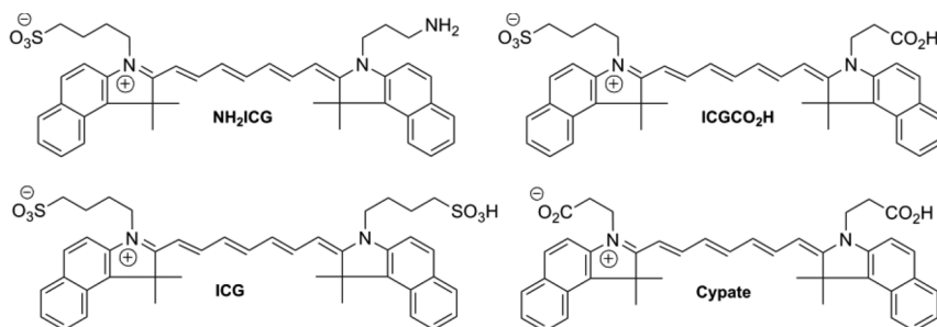
Fig. 1 Chemical structures of NH 2 -ICG and structural comparison with its analogs ICG-CO 2 H, ICG, and cypate.
