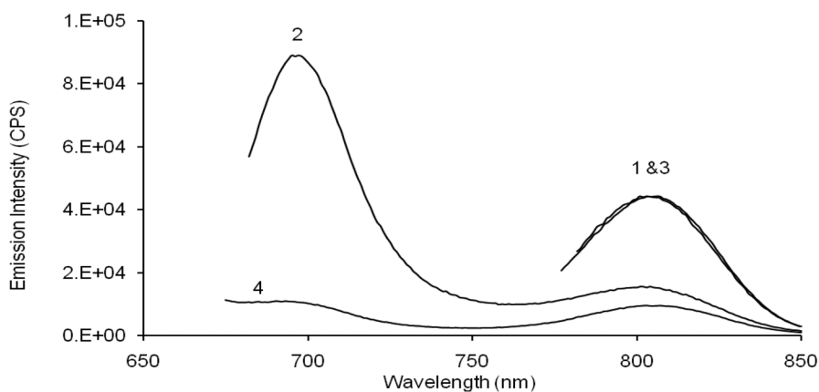
Fig. 4 Comparative emission spectra of \text{NH}_2\text{-ICG} and ICG excited 20 nm and 120 nm below \lambda_{\text{max}}^{\text{abs}} . Emission of ICG at \lambda_{\text{max}}^{\text{abs}}-20 nm excitation (curve 3) is normalized to the same intensity of emission of \text{NH}_2\text{-ICG} on \lambda_{\text{max}}^{\text{abs}}-20 nm excitation (curve 1). For comparative purpose, emission of ICG at \lambda_{\text{max}}^{\text{abs}}-120 nm excitation (curve 4) is normalized by the same factor as in the normalization of the emission at \lambda_{\text{max}}^{\text{abs}}-20 nm excitation. Curve 2 is \text{NH}_2\text{-ICG} emission at \lambda_{\text{max}}^{\text{abs}}-120 nm excitation.
