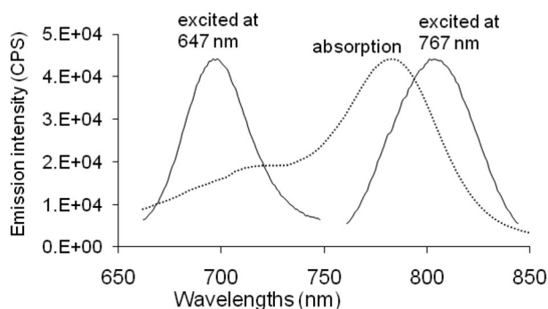
Fig. 2 Absorption and emission spectra of NH 2 -ICG in 20 % aq. dimethyl sulfoxide (DMSO). Absorption and shorter wavelength emission curves are normalized to the same intensity of the principal emission band. Emission taken at absorbance of A = 0.10 at \lambda_{\text{max}}^{\text{abs}} . The actual shorter wavelength emission intensity is comparable to the principal emission at the optimal excitation wavelength.
