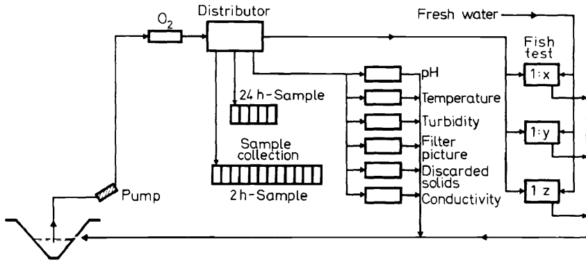
Figure 20. Monitoring system.
