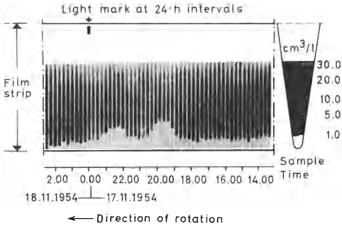
Figure 13. Automatic measuring and recording of sludge content on a film strip.
