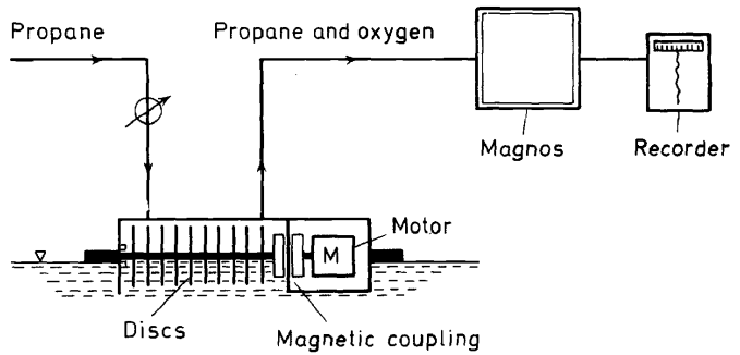
Figure 16. Oxygen measurement using phase exchanger type 'B'.
