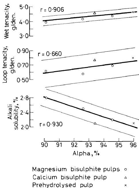
Figure 3. Wet tenacity, loop tenacity and alkali solubility of Polynosic fibres plotted against the alpha contents of the pulps [O, Magnesium bisulphite pulps; Δ, calcium bisulphite pulp; ×, prehydrolysed pulp]
