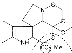
Malonate unit
