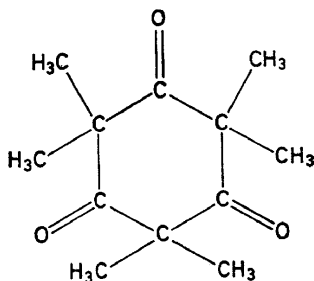
Figure 9. Cyclic trimer of dimethylketene
